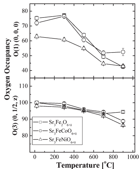
Figure 4. Variation of the occupancy factor of the O(1) ( 2a, 0, 0, 0 ) and O(3) ( 8g, 0, 1/2, z ) crystal sites with temperature in air.
