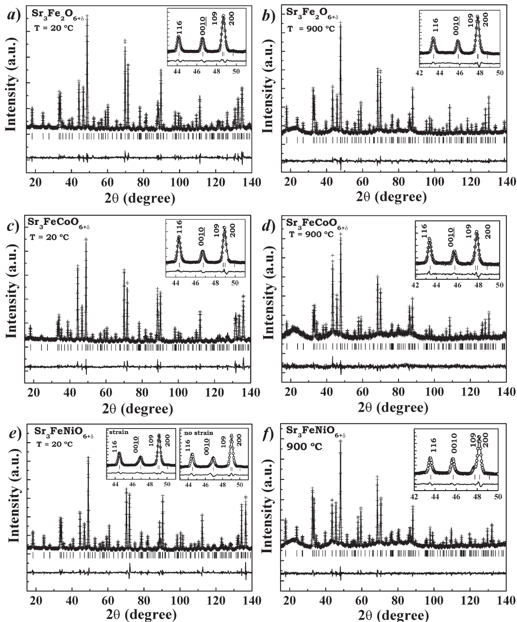
Figure 2. Powder neutron diffraction patterns of \text{Sr}_3\text{FeMO}_{6+\delta} ( M = \text{Fe}, \text{Co}, \text{Ni} ) at room temperature (a, c, and e) and at T = 900^\circ\text{C} (b, d, and f) in air. Every figure includes the observed data (+), the calculated data (solid line), the difference plot (bottom), and the allowed reflections (marks) for the I4/mmm space group. The insets expand the 2\theta range 42^\circ \leq 2\theta \leq 50^\circ to appreciate in more detail the quality of the refinements. The inset in panel “e” shows the refinements when the strain model for \text{Sr}_3\text{FeNiO}_{6+\delta} at room temperature is considered and when it is neglected. The quality of the refinement improves when the strain model is included (see text).
